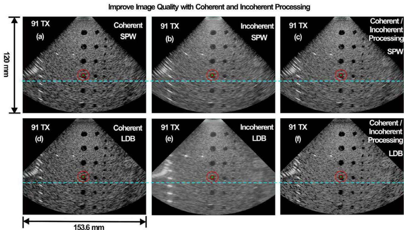
Figure 3. Images obtained with the coherent superposition ((a) and (d)), incoherent superposition ((b) and (e)), and the new coherent and incoherent processing ((c) and (f)) using 91 sub-images (corresponding to 91 transmissions or 91 TX) reconstructed with the steered plane wave (SPW) ((a), (b), and (c)) and limited-diffraction-beam (LDB) ((d), (e), and (f)) methods. The threshold for (c) and (f) is 3.16 for the ratio image. The Fourier-based method were used to reconstruct all images [1][2][4][5]. (The results of coherent and incoherent superposition are similar to those of [17].)
