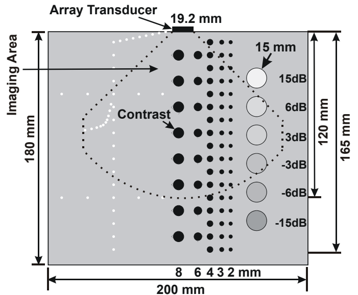
Figure 1. A cross-section of an ATS539 tissue-mimicking phantom showing the imaging areas of 120 mm depth with \pm 45 degree field of view for the experiments. (Modified from Fig. 4 of [18].)
